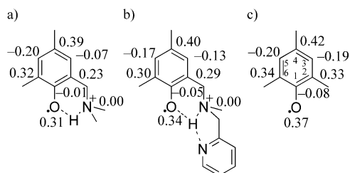
Scheme 4. Spin density in a) single hydrogen bonded phenoxyl-radical model system b) bifurcated hydrogen bonded phenoxyl-radical model system and c) “free” 2,4,6 tri(methyl)phenoxyl radical.
