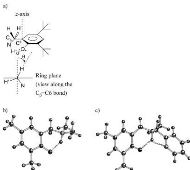
Figure 3. a) Model for the hydrogen bonded phenoxyl radicals; b) (U)B3LYP6-31g* optimized structure of a single hydrogen bonded phenoxyl-radical model system; c) (U)B3LYP6-31g* optimized structure of a bifurcated hydrogen bonded phenoxyl-radical model system.
