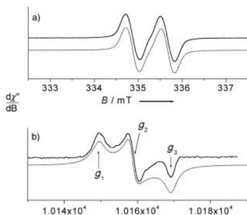
Figure 2. EPR spectra of electrochemically oxidized \text{HL}^{\text{Benz}\cdot+} radical species recorded in \text{CH}_2\text{Cl}_2 solution (0.1 M TBAP): a) isotropic X-band spectrum at 213 K (modulation: 100 KHz, 0.0393 mT, Frequency: 9.4103 GHz, 10 mW, [\text{HL}^{\text{Benz}\cdot+}] = 1.6 \text{ mM} ); b) 285 GHz spectrum at 5 K ( [\text{HL}^{\text{Benz}\cdot+}] = 5 \text{ mM} ); solid lines: experimental spectrum, dotted lines: simulation by using the parameters given in the Supporting Information. ( B = magnetic-flux density).
