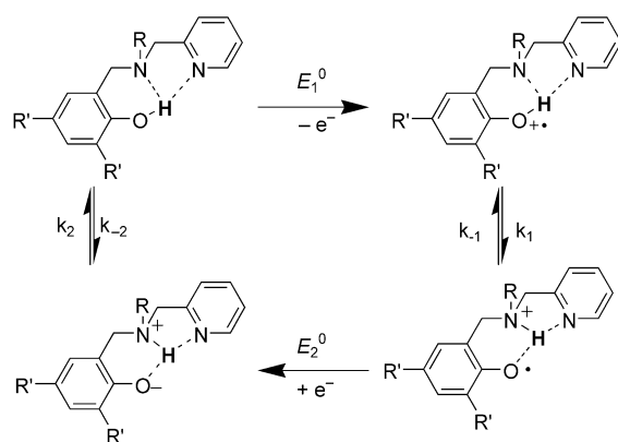
Scheme 2. Minimum proton-migration process during electron transfer; K_1 = k_1/k_{-1} and K_2 = k_2/k_{-2} .
