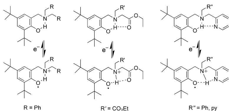
Scheme 1. Phenol derivatives \text{HL}^{\text{Benz}} ( R = \text{Ph} ), \text{HL}^{\text{est}} ( R' = \text{CO}_2\text{Et} ), \text{HL}^{\text{Benzpy}} ( R'' = \text{Ph} ) and \text{HL}^{\text{py}} ( R'' = \text{py} ) and their corresponding hydrogen-bonded phenoxyl radicals.
