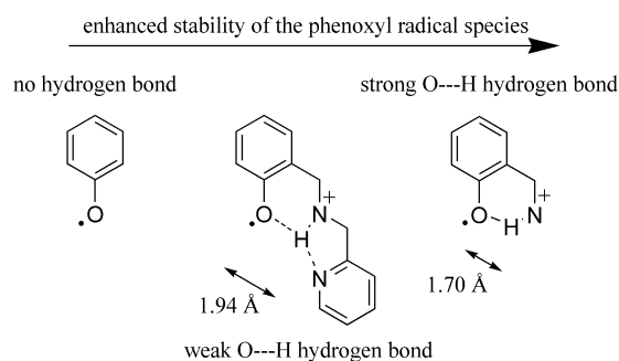
Scheme 3. Stability of phenoxyl radical species (O–H distances were obtained from DFT calculations, see text) under our experimental conditions.
