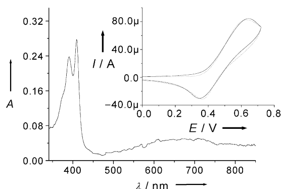
Figure 1. Electronic spectrum of the electrogenerated \text{HL}^{\text{Benz}+} 0.32 mM recorded in \text{CH}_2\text{Cl}_2 0.01 M TBAP at 233 K (path length l = 1 cm); Inset: CV curve of \text{HL}^{\text{Benz}} , 2.4 mM in \text{CH}_2\text{Cl}_2 0.1 M TBAP at 298 K; Scan rate: 0.1 \text{Vs}^{-1} , solid line: experimental, dotted line: simulation by using the parameters given in the text. ( A = absorption, arbitrary units; l = electrical current).
